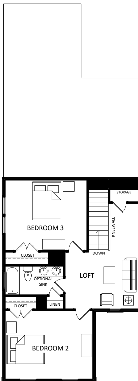
SECOND FLOOR
